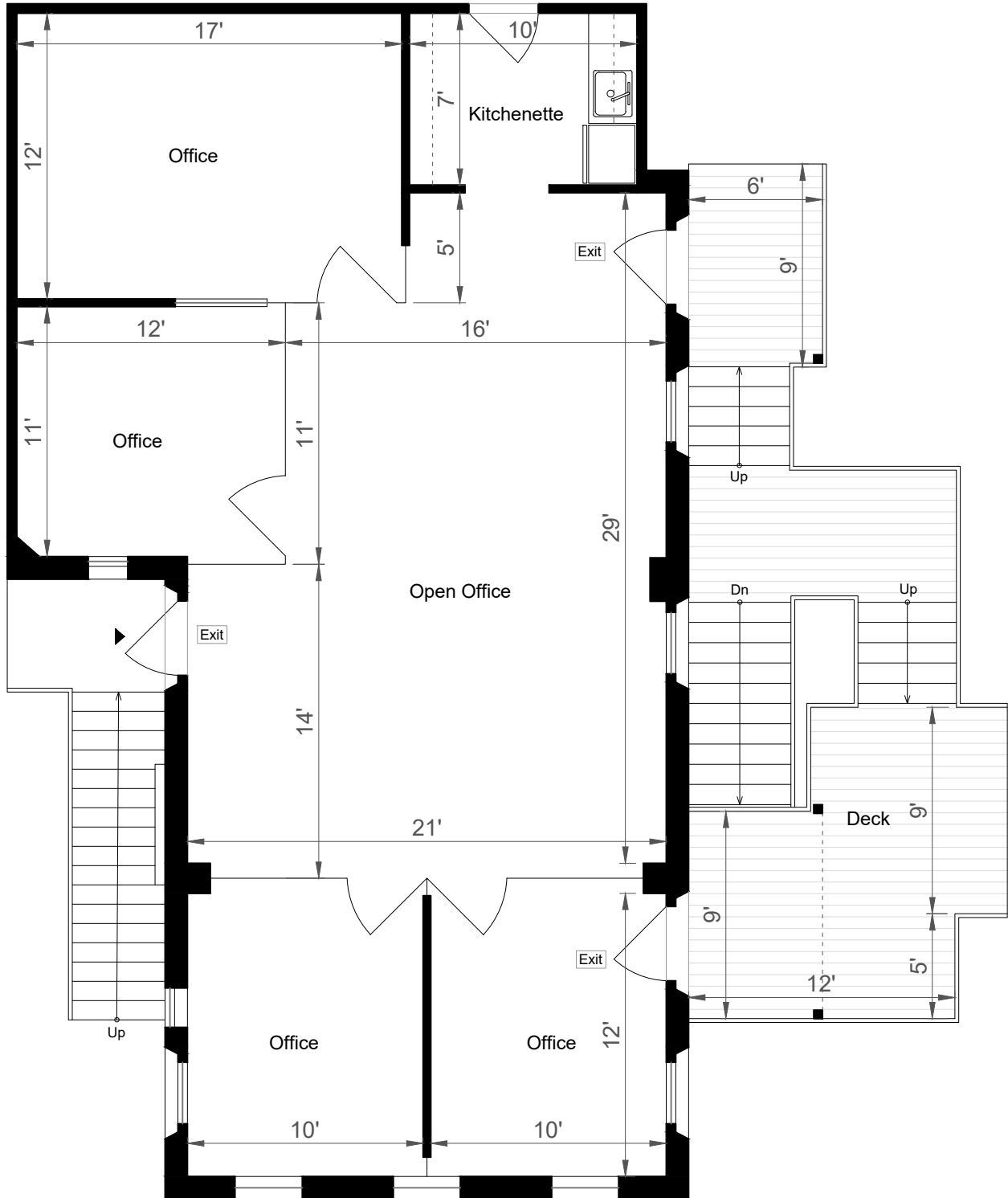
FLOOR PLAN
